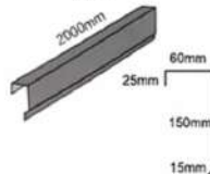
Barge Board Cover 山墙板
