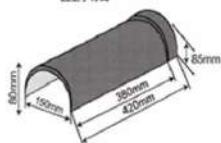
Circular Ridge Cap 圆型小脊瓦
